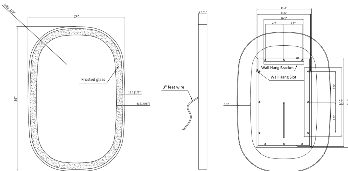
LEFT VIEW
