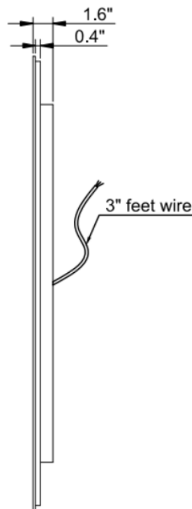
LEFT VIEW
